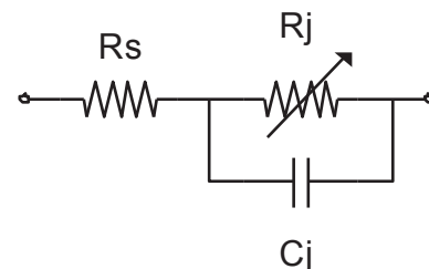
Electrical equivalent model of a PIN diode (die only, no package parasitics)
