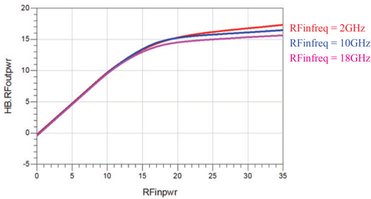
Pin versus Pout of the symmetrical 5th order limiter at 2, 10 and 18GHz
