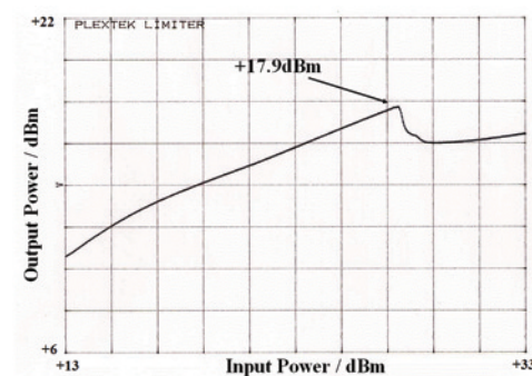
Measured Pin versus Pout from a previous Plextek RFI limiter design
