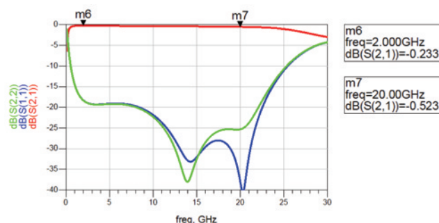
Small-signal low loss performance of the high-power (asymmetrical) 5th order limiter
