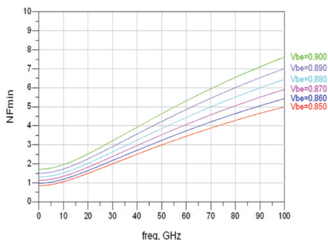
NF_{min} versus frequency for different bias points, SG25H3 transistor
