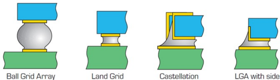
Examples of LTCC to PCB interconnects (DT Microcircuits)
